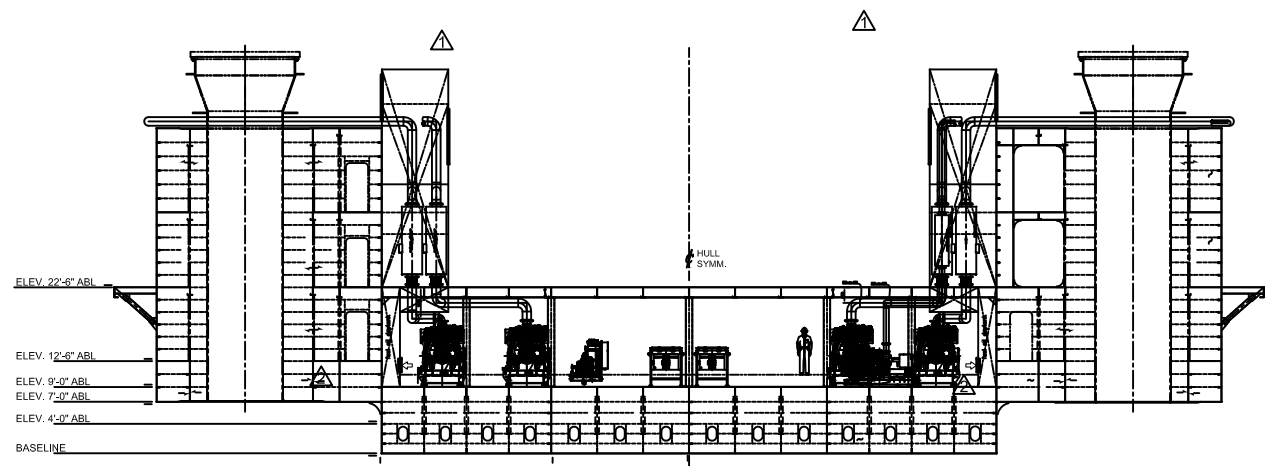
TRANSVERSE ELEVATION AT FR. 2 LOOKING AFT
