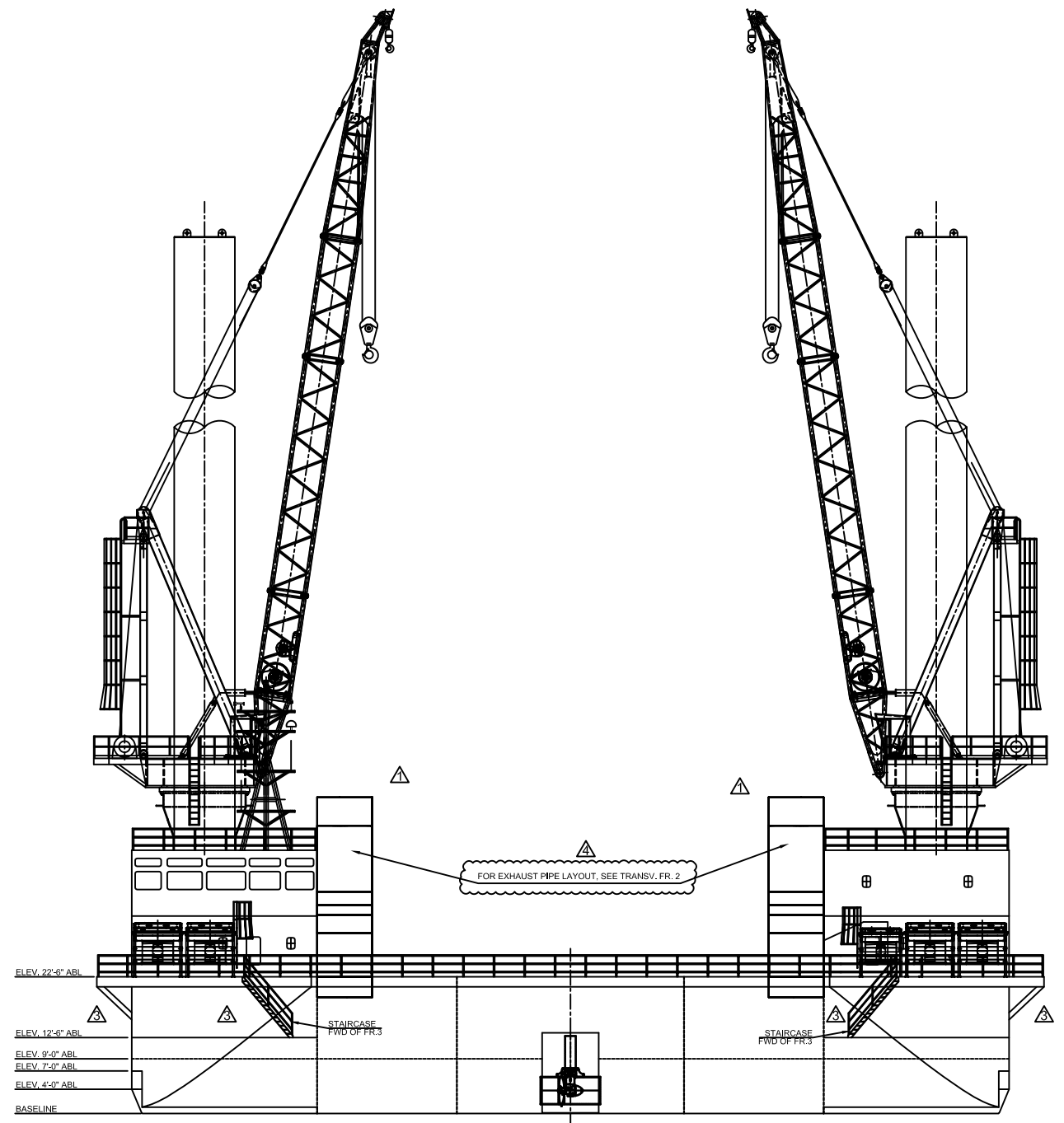
BOW ELEVATION LOOKING AFT
